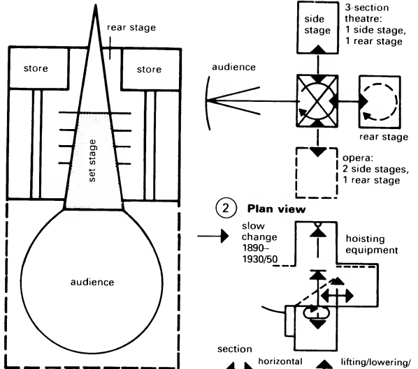
① Scene-changing technology, classical stage system of the 18th and 19th centuries
